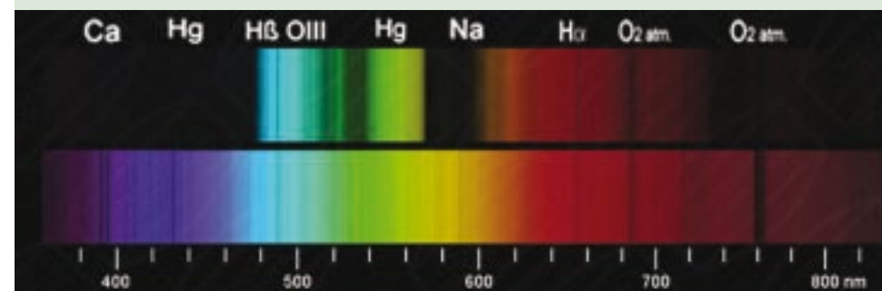
Image 4 - Contrast-Booster spectrum above the solar spectrum.
