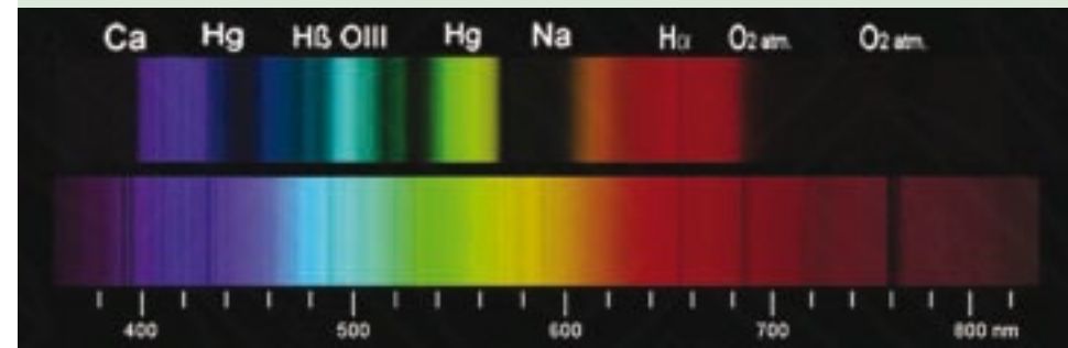
Image 3 - Spectrum of the Baader Neodymium Moon & Skyglow filter above the solar spectrum.
